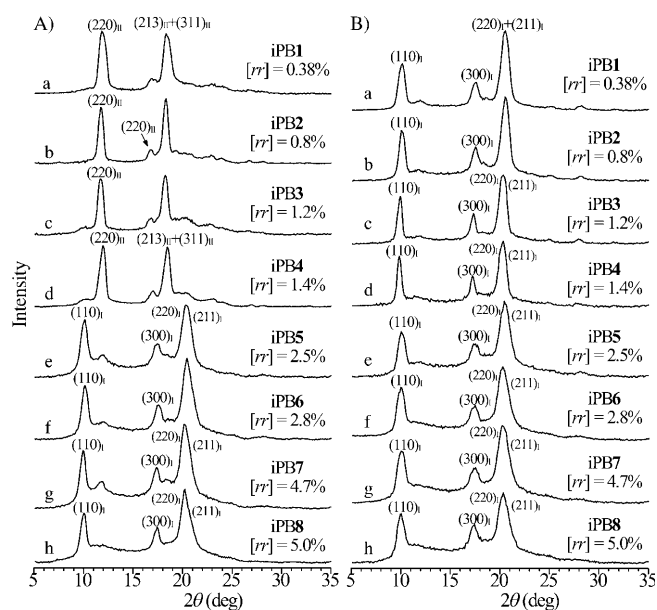
Figure 2. X-ray powder diffraction profiles of samples of iPB of different stereoregularity crystallized by cooling the melt to room temperature (or lower temperature) at a cooling rate of 2.5^\circ\text{C min}^{-1} recorded soon after the cooling (A) and after aging at room temperature for at least 1 month (B). The (110)_I , (300)_I , and (220)_I + (211)_I reflections of form I at 2\theta = 9.9 , 17.3, and 20.5°, respectively, and the (200)_{II} , (220)_{II} , and (213)_{II} + (311)_{II} reflections of form II at 2\theta = 11.9 , 16.9, and 18.3°, respectively, are indicated. All spectra are vertically displaced.
